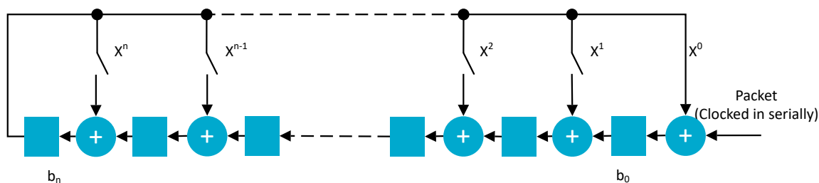
Figure 113: n bit CRC generation
