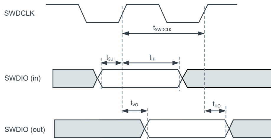
Figure 194: SWD timing diagram
