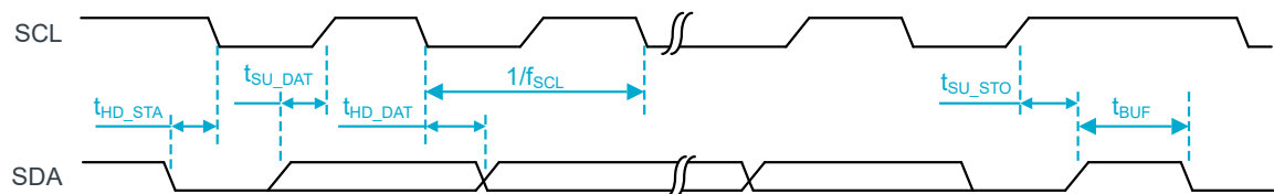
Figure 196: TWIS timing diagram, 1 byte transaction
