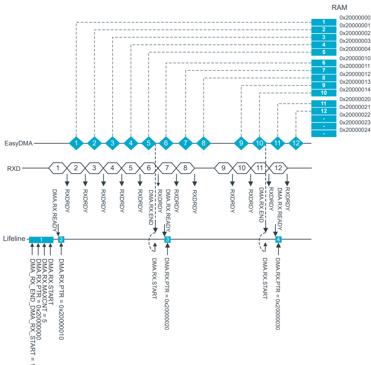
Figure 160: UARTE reception
