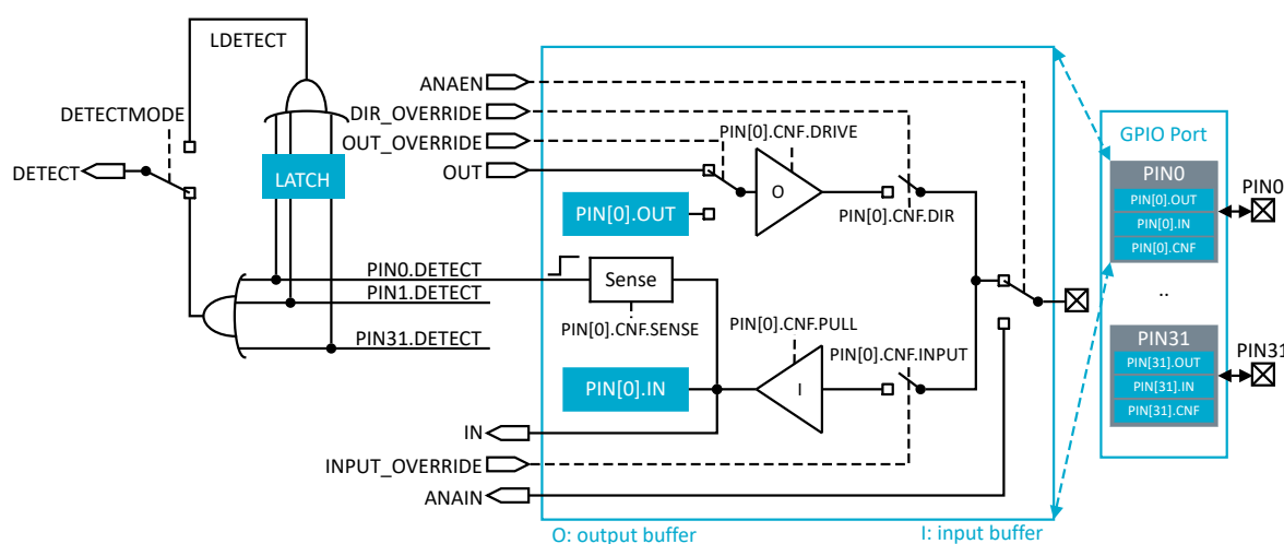
Figure 60: GPIO port and the GPIO pin details
