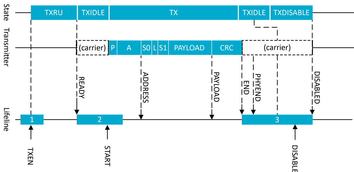
Figure 115: Transmit sequence
