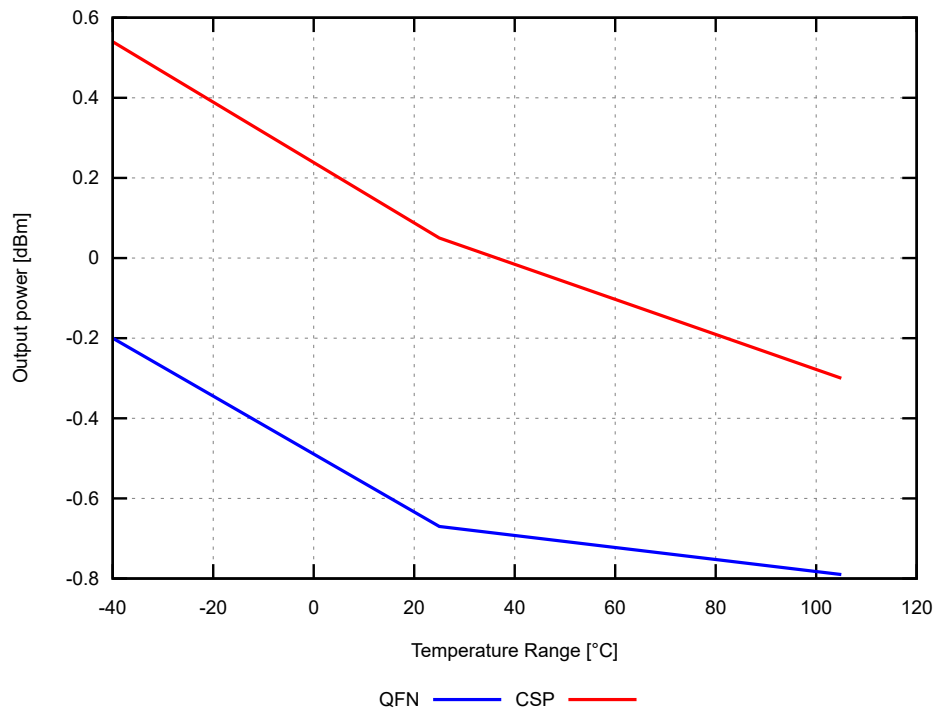
Figure 186: Output power, 1 Mbps Bluetooth low energy mode, at 0 dBm setting (typical values)
