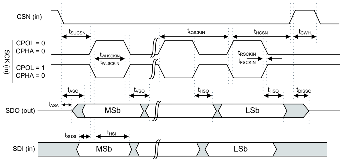
Figure 191: SPIS timing diagram, CPHA = 0
