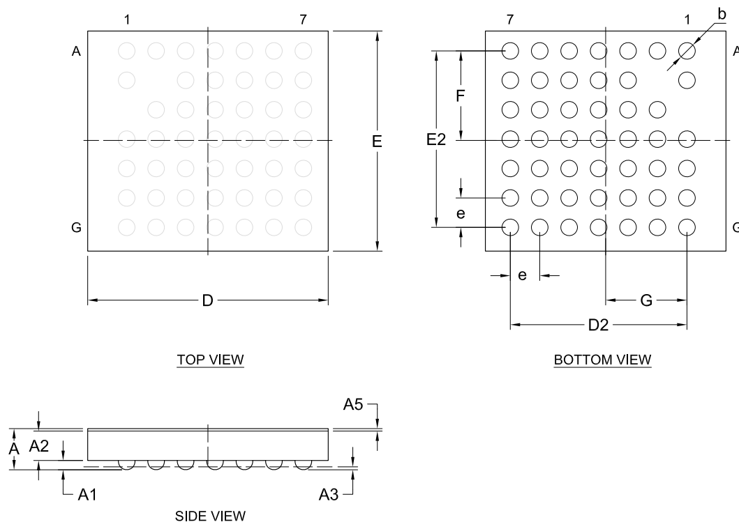
Figure 174: Package dimensions in millimeters
