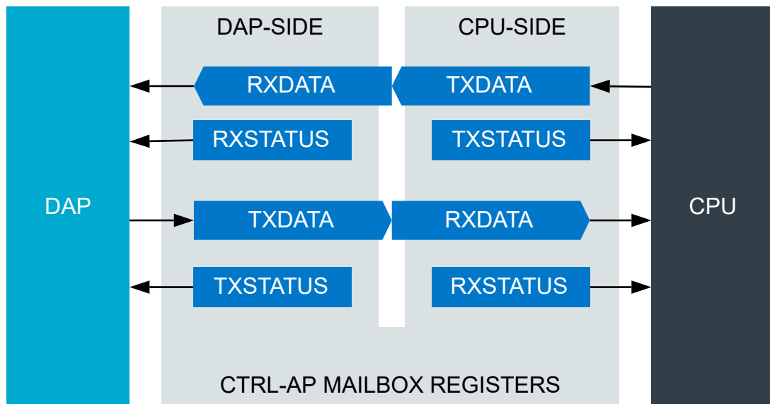
Figure 170: Mailbox register interface
