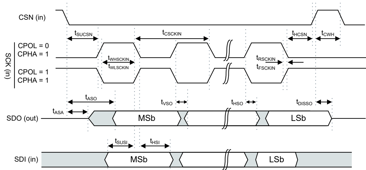
Figure 192: SPIS timing diagram, CPHA = 1
