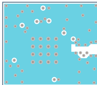
Figure 180: Mid layer 2
