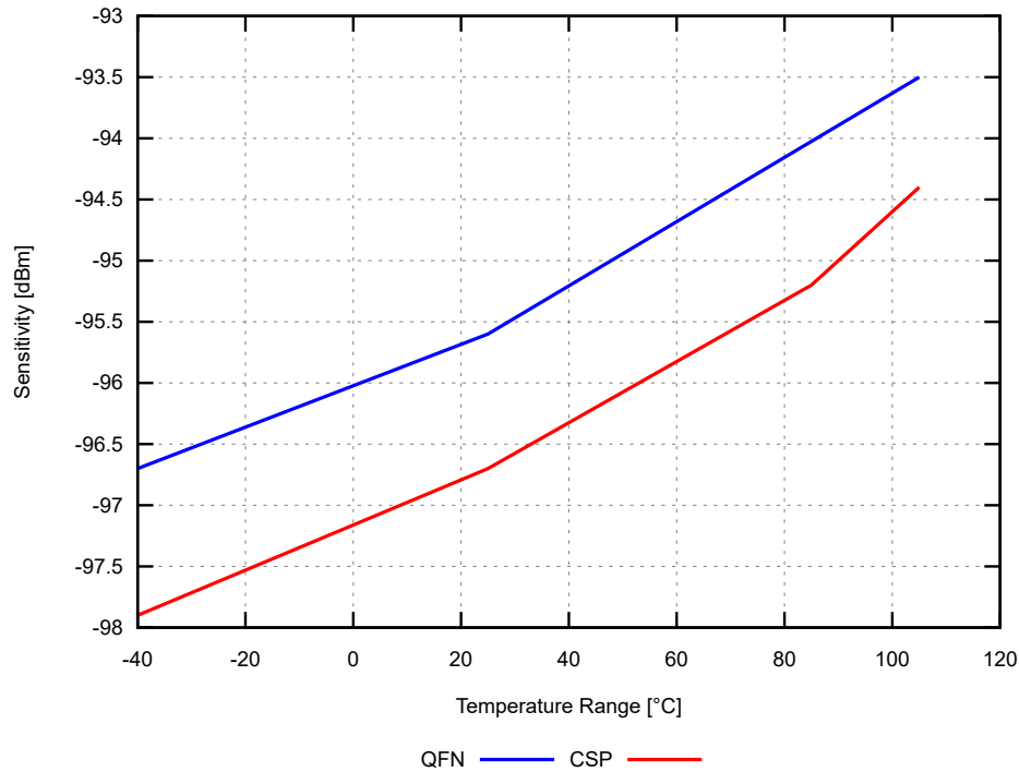
Figure 187: Sensitivity, 1 Mbps Bluetooth LE ideal transmitter, packet length \leq 37 bytes BER = 1E-3 (typical values)
