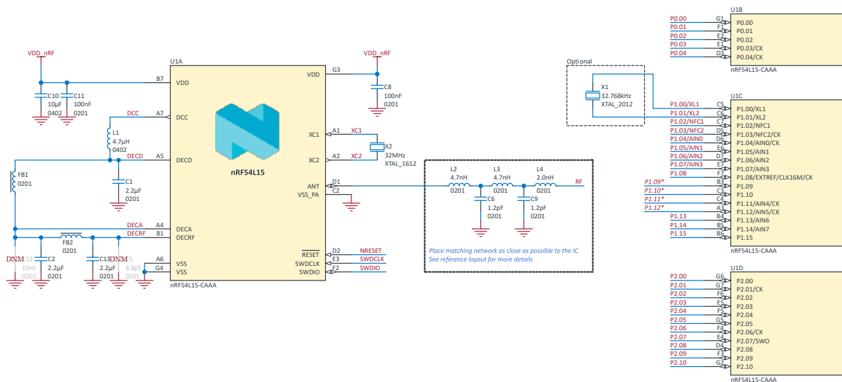
Figure 176: Circuit configuration 1 schematic
