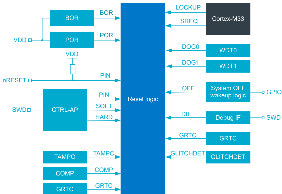
Figure 22: Reset sources
