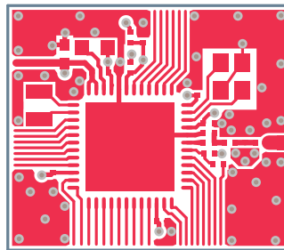
Figure 178: Top layer
