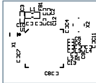
Figure 177: Top silk layer
