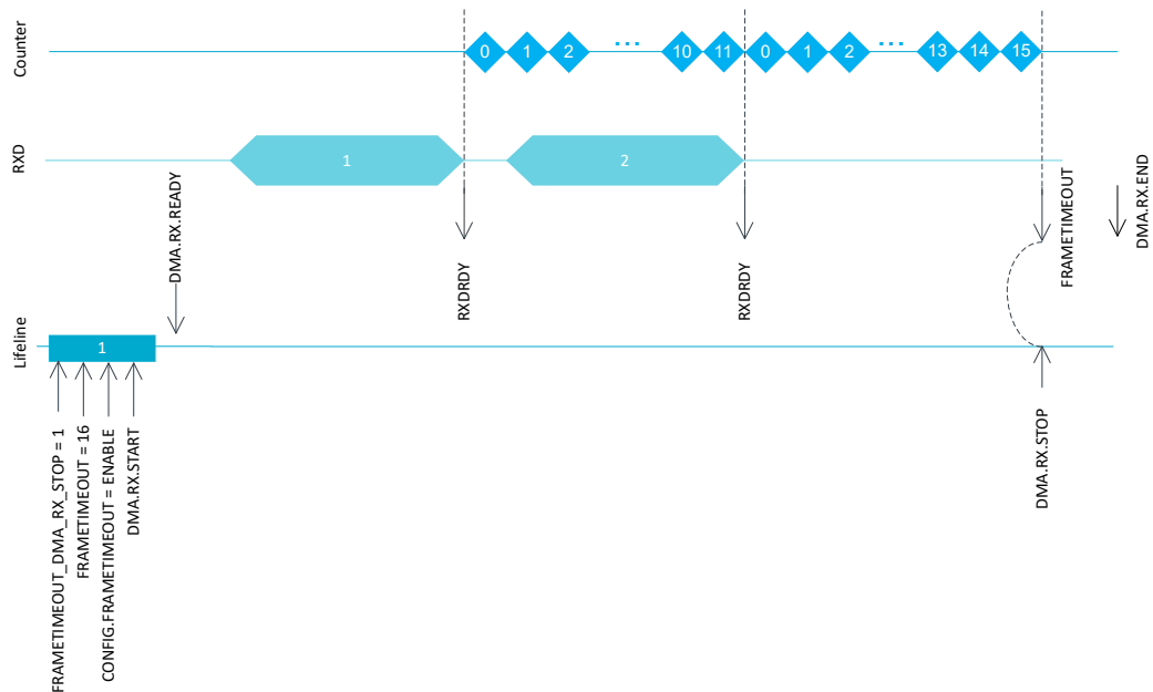
Figure 163: UARTe reception frame timeout
