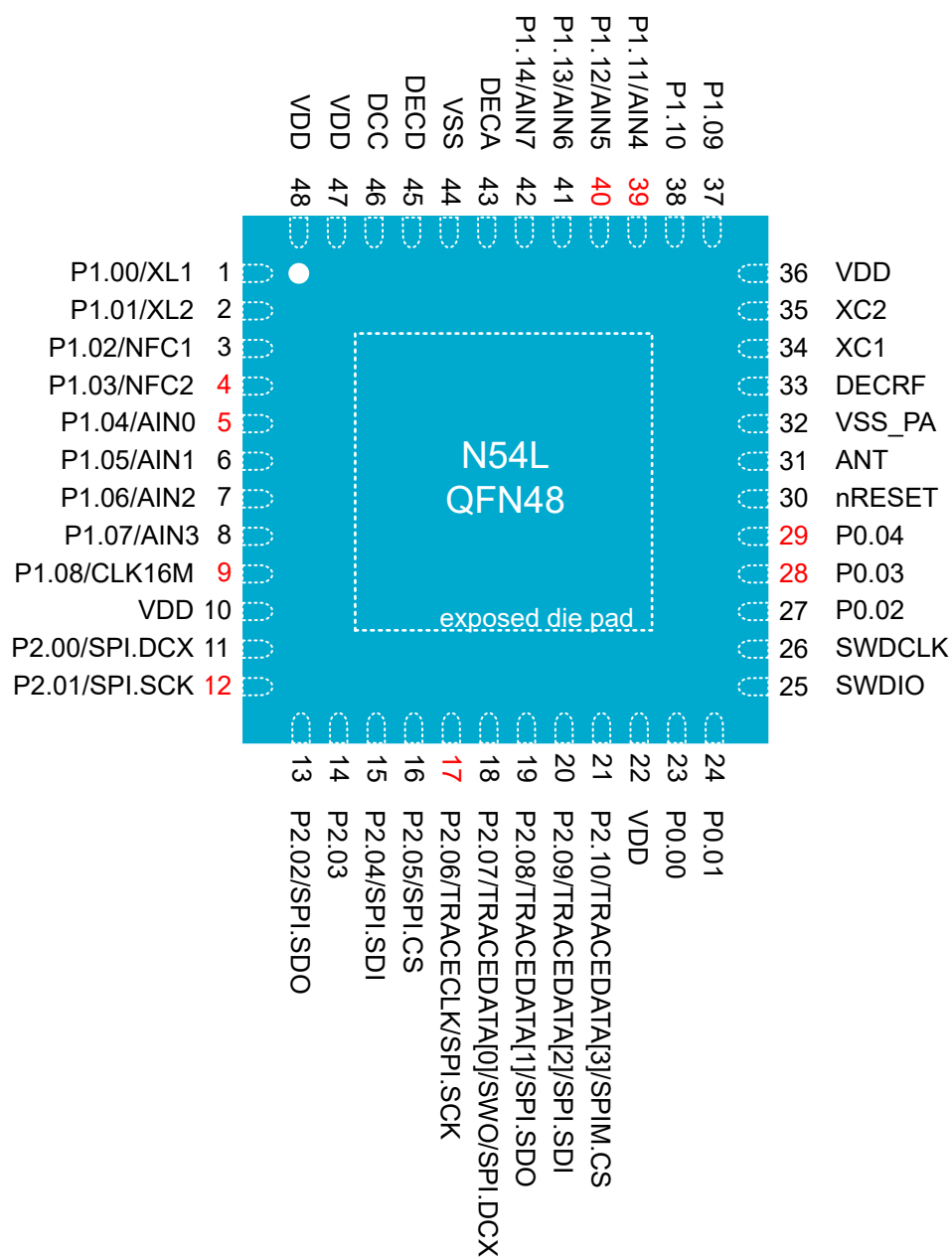
Figure 171: QFN48 pin assignments, top view
