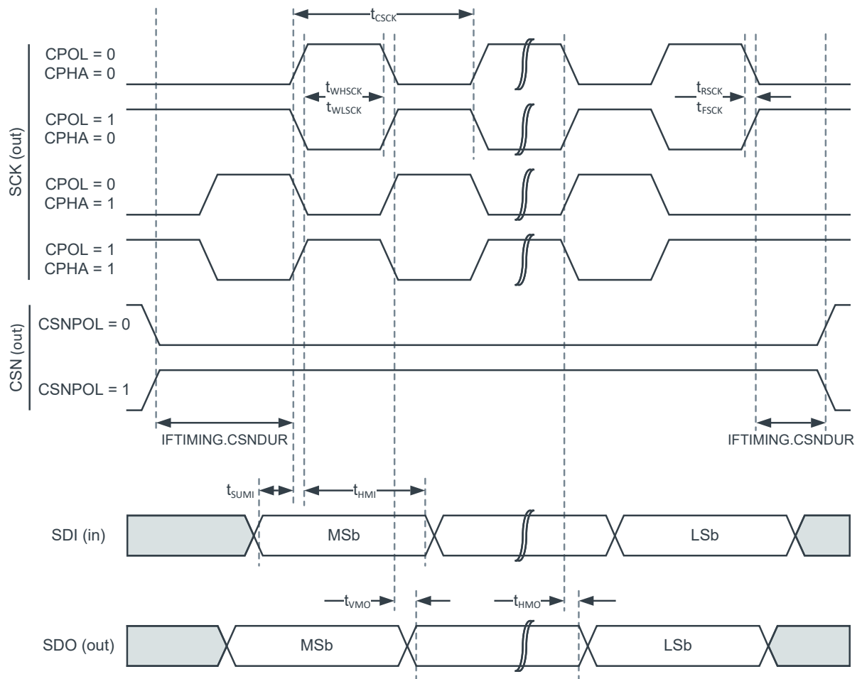
Figure 190: SPIM timing diagram
