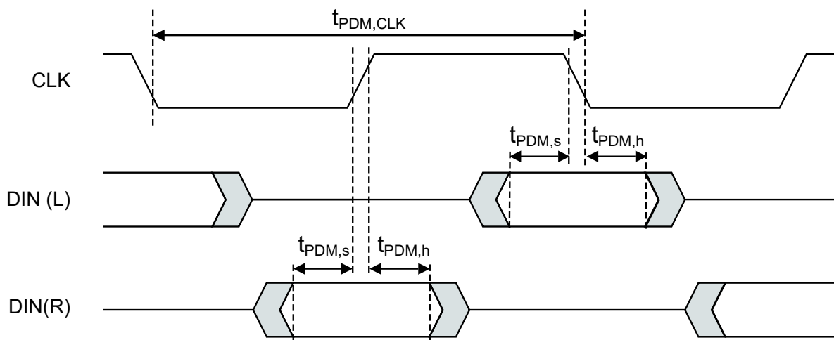
Figure 184: PDM timing diagram
