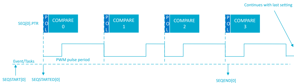
Figure 102: Simple sequence example
