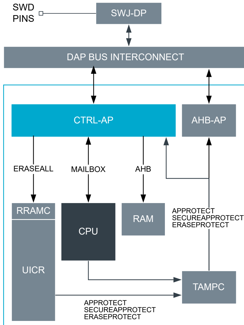
Figure 168: Control access port details
