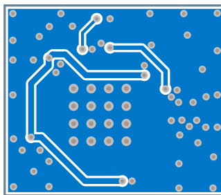
Figure 181: Bottom layer
