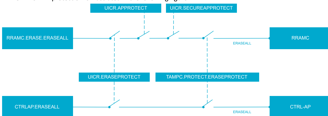
Figure 166: ERASEALL protection overview
