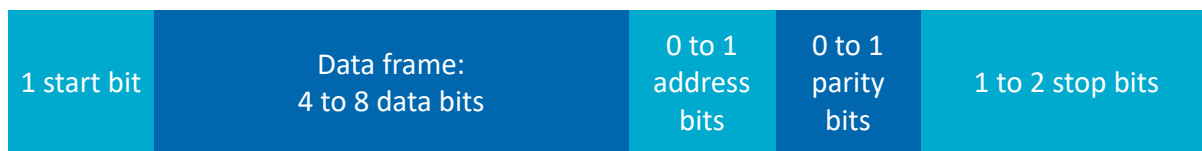
Figure 162: UARTE frame
