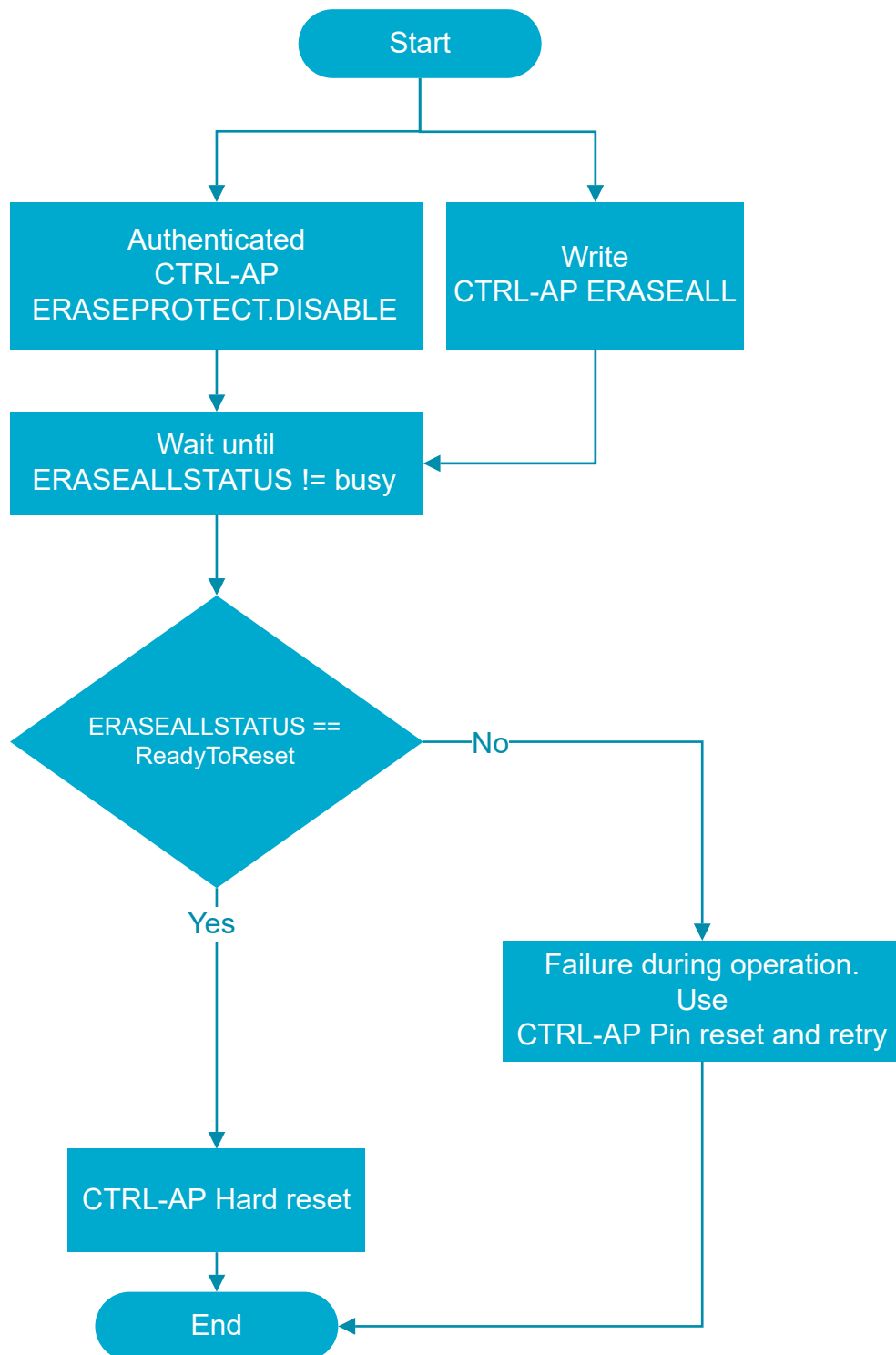
Figure 169: Erase all states
