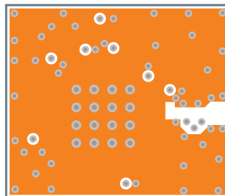
Figure 179: Mid layer 1
