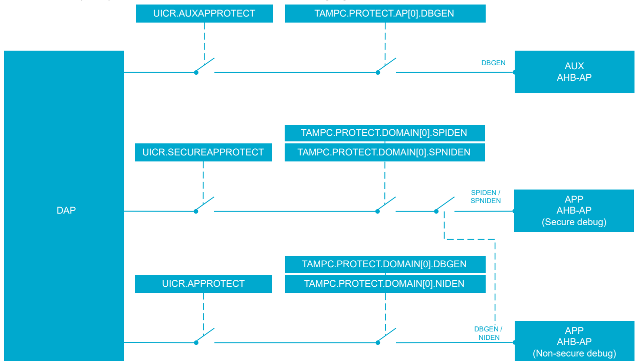
Figure 165: Access port protection overview
