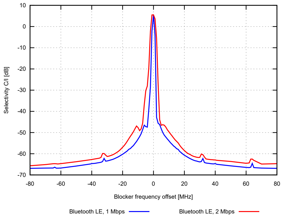
Figure 188: Selectivity Bluetooth Low Energy (Typical performance; wanted signal at channel 2440 MHz and -67 dBm input level)
