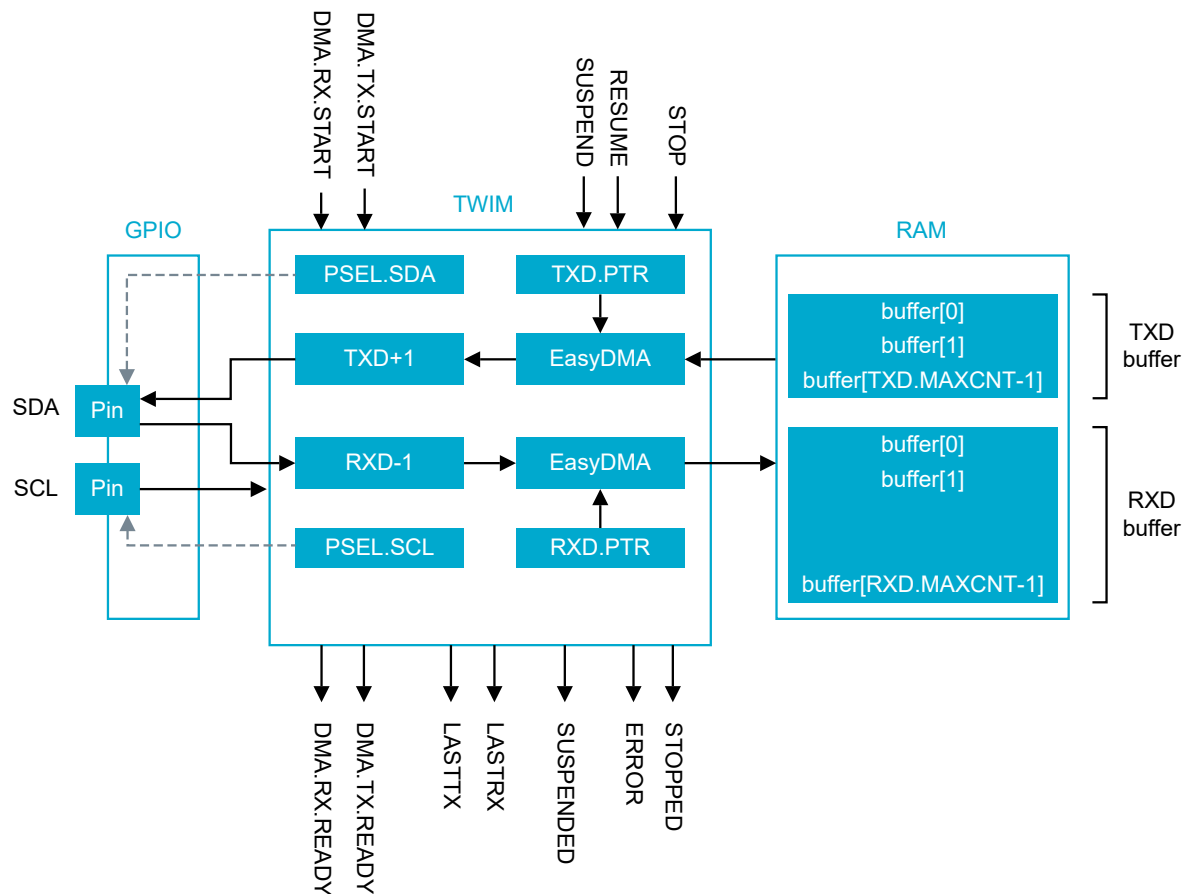
Figure 144: TWIM with EasyDMA
