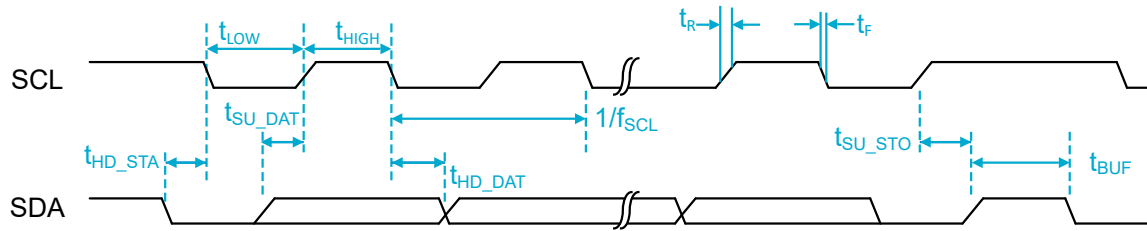
Figure 195: TWIM timing diagram, 1 byte transaction
