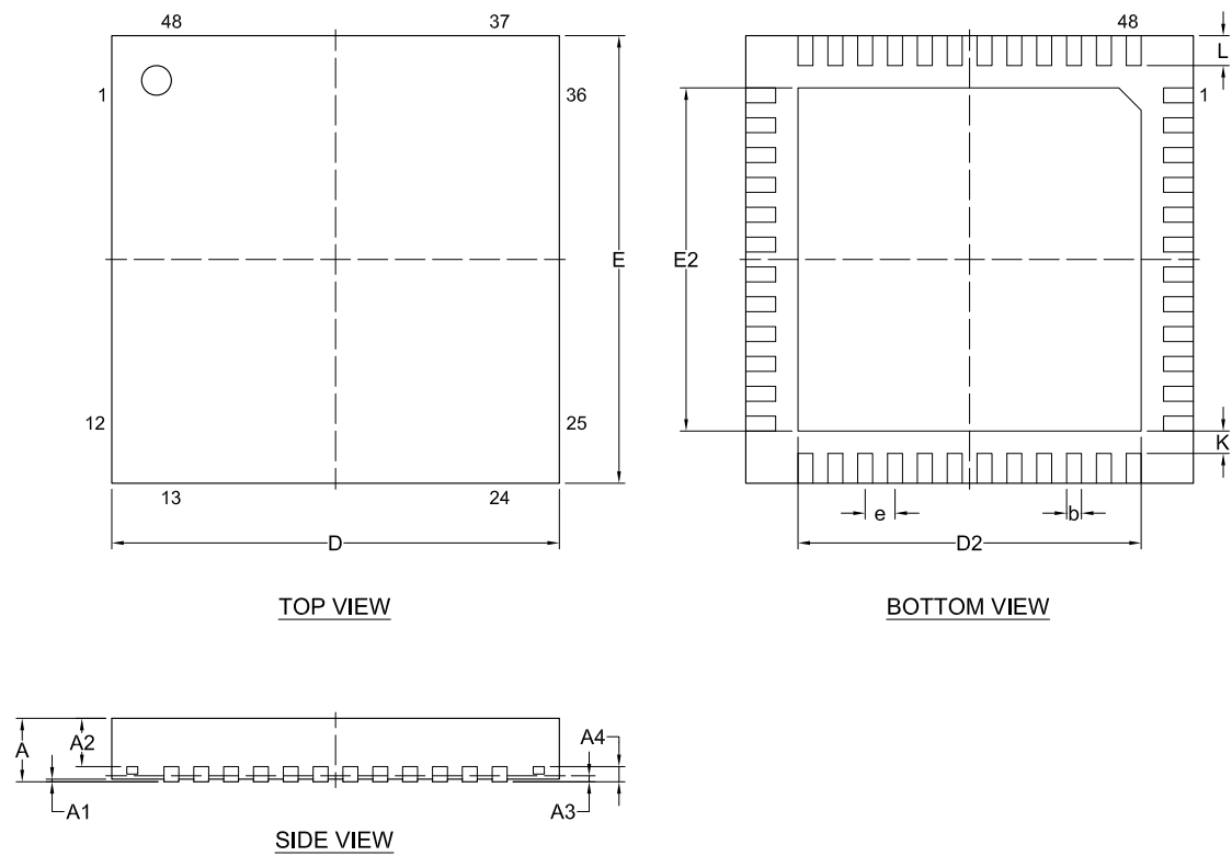
Figure 173: QFN48 6x6 mm package
