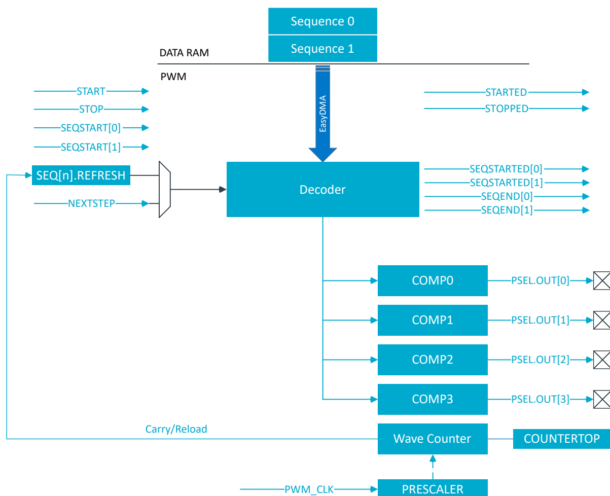
Figure 98: PWM module
