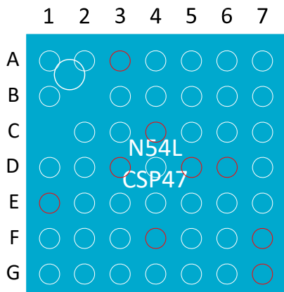
Figure 172: CSP47 pin assignments, top view
