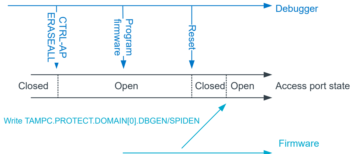
Figure 167: Access port unlocking
