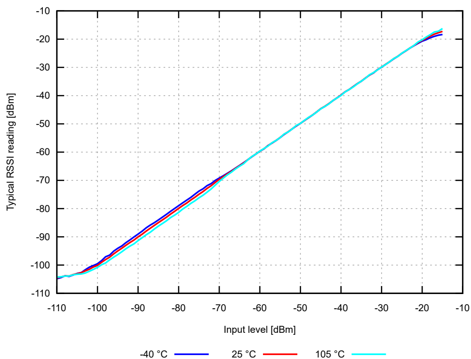
Figure 189: RSSI reading versus input level. Typical values.
