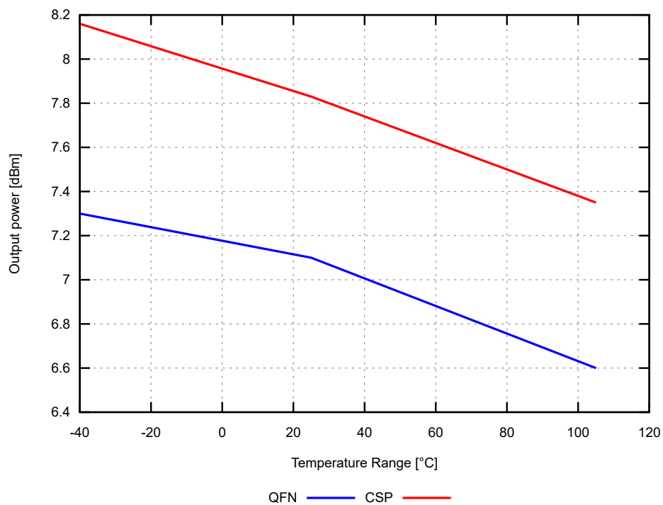
Figure 185: Output power, 1 Mbps Bluetooth low energy mode, at maximum TXPOWER setting (typical values)
