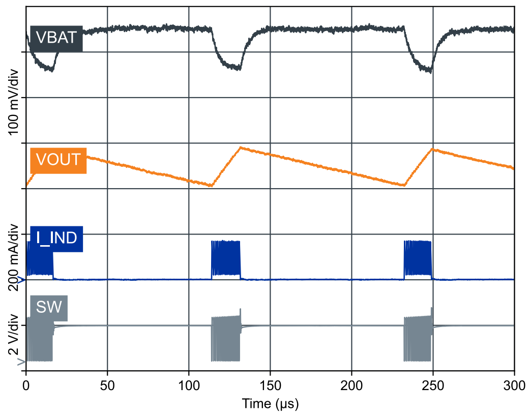
Figure 25: V_{OUT}=1.8 V: Switching waveforms in Ultra-low power mode (load=10 mA)
