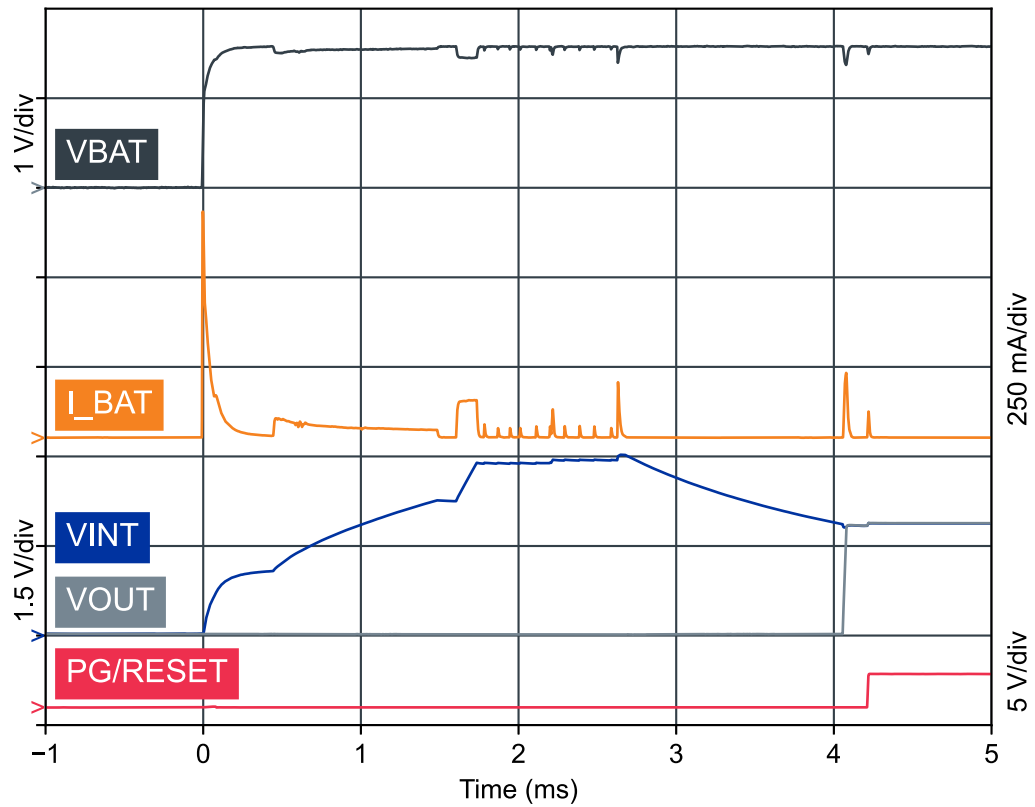
Figure 10: Battery (alkaline AA) insertion, V_{SET} connected to ground
