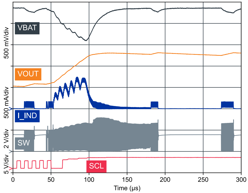
Figure 20: Output voltage programming via TWI from 1.8 V to 2.5 V in Auto mode (LDOSW in High power mode, no load)
