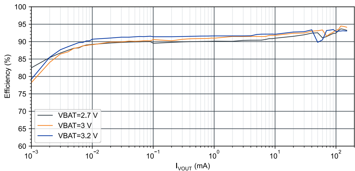
Figure 7: V_{OUT}=3.3 V: Auto mode efficiency
