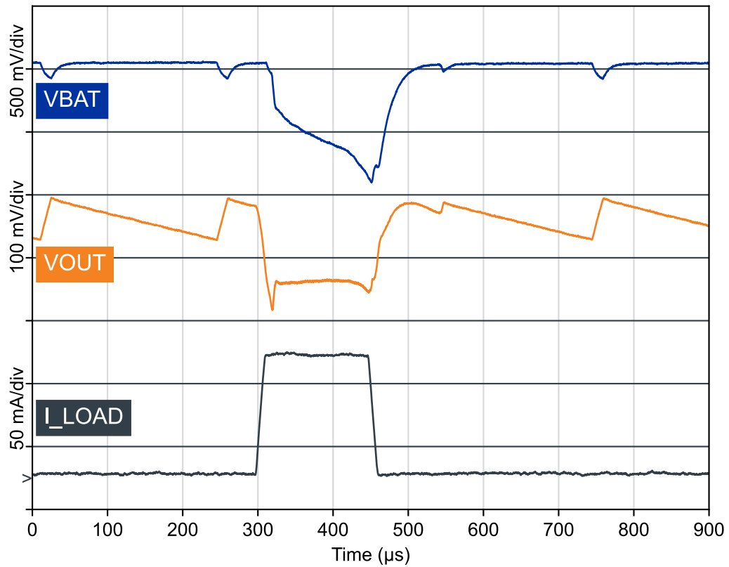
Figure 16: V_{OUT}=3.0\text{ V} : Auto mode load transient from 1 mA to 100 mA in 10 \mu\text{s} (automatic mode change from Low power mode to High power mode, and back)
