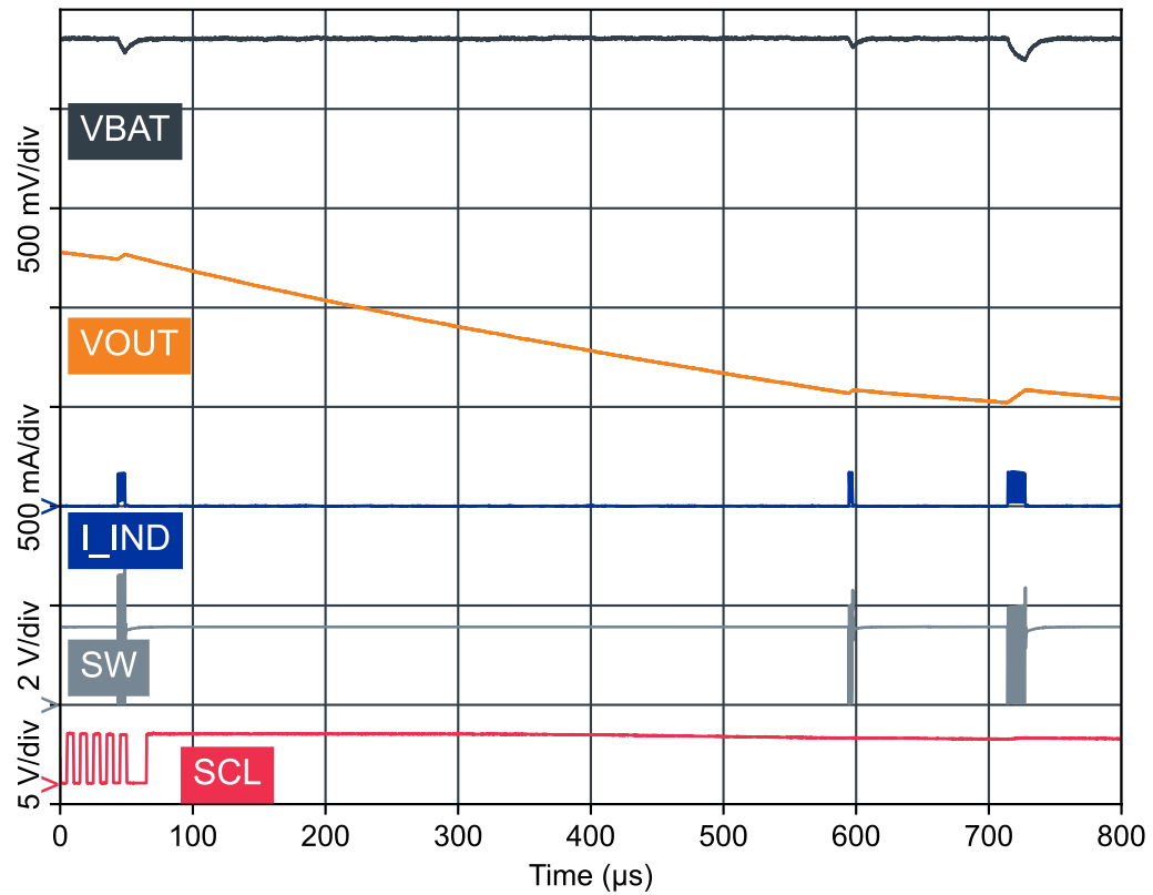
Figure 22: Output voltage programming via TWI from 2.5 V to 1.8 V in Low power mode (LDOSW in High power mode, no load)
