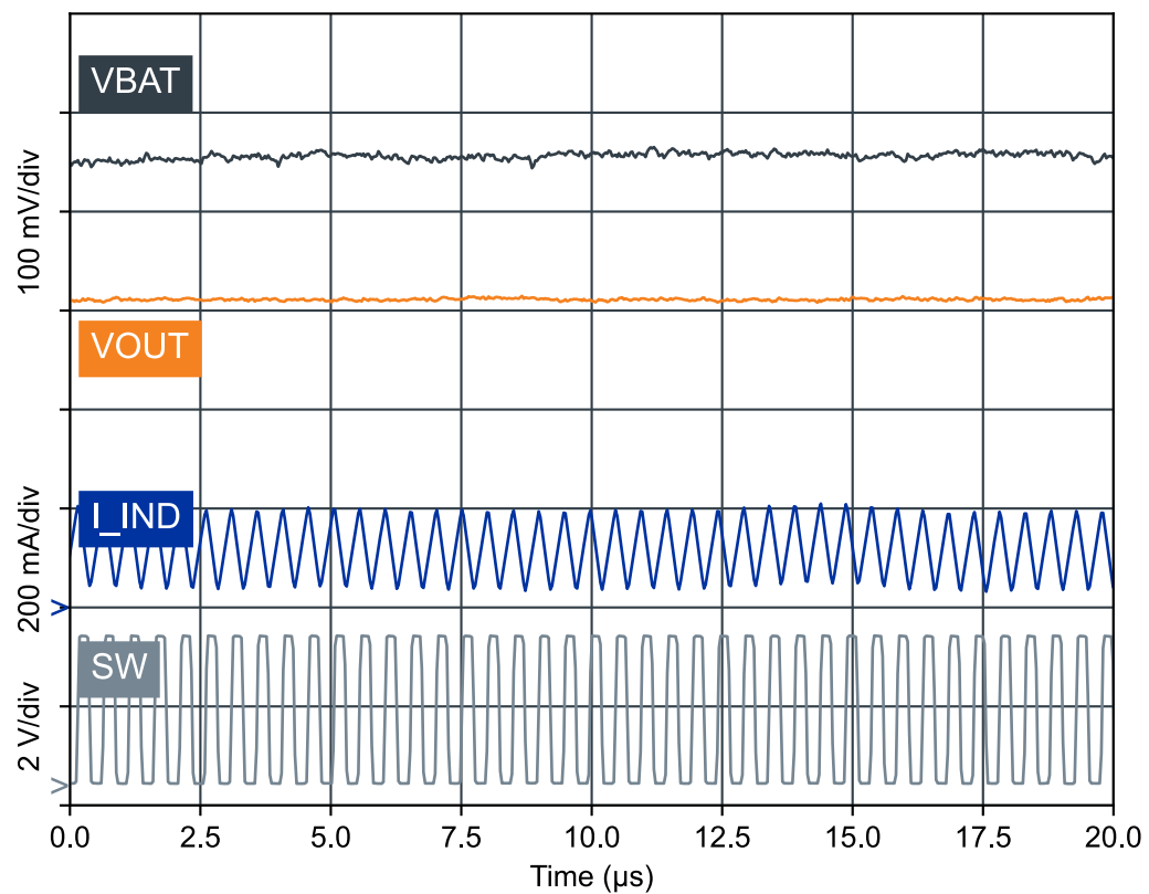
Figure 23: VOUT=3.0 V: Switching waveforms in High power mode (load=50 mA)
