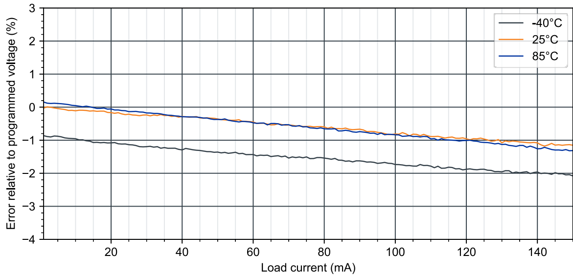
Figure 12: V_{OUT}=3.0 V: High power mode load regulation ( V_{BAT}=2.5 V)
