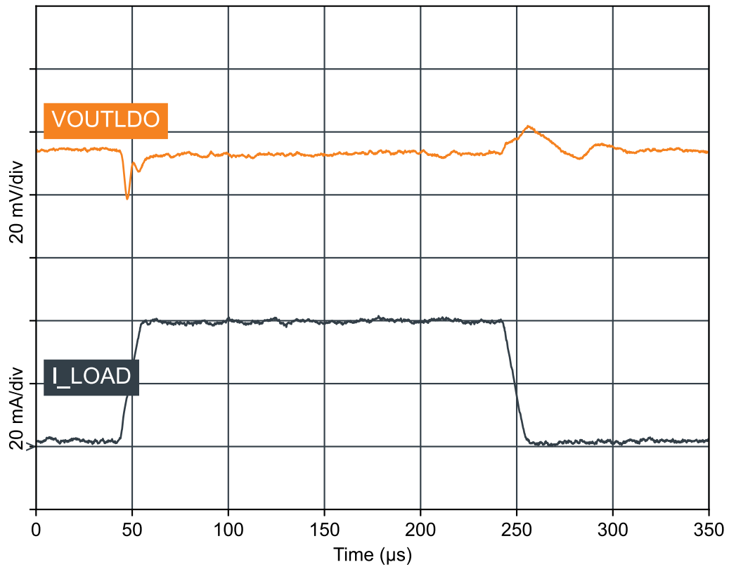
Figure 35: V_{OUTLDO}=1.8\text{ V} : High power mode LDO load transient from 1 mA to 40 mA in 10 μs ( V_{INT}=3.0\text{ V} )
