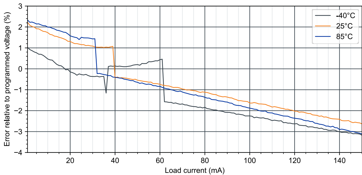
Figure 13: V_{OUT}=1.8 V: Auto mode load regulation ( V_{BAT}=1.5 V)
