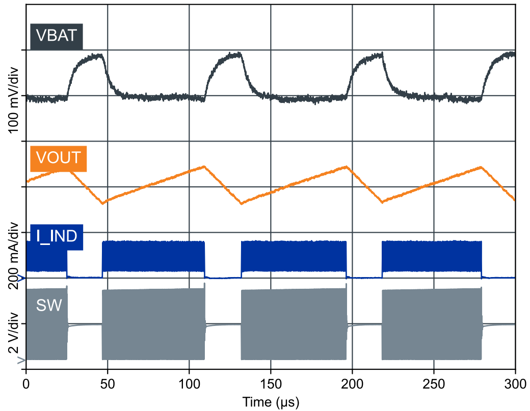
Figure 24: V_{OUT}=3.0 V: Switching waveforms in Low power mode (load=30 mA)
