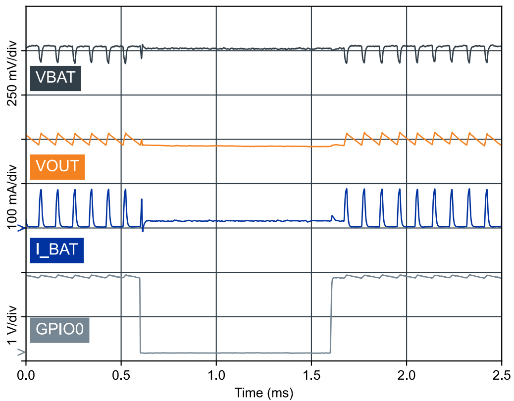
Figure 19: V_{OUT}=1.8 V: Mode change from Low power mode to High power mode using GPIO control (load=10 mA)
