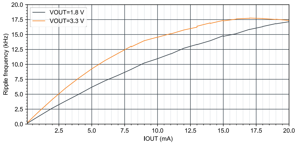
Figure 26: Low power mode VOUT ripple frequency vs. load (VBAT=1.5 V)
