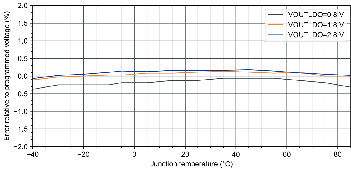
Figure 33: V_{OUTLDO}=1.8\text{ V} : Ultra-low power mode LDO accuracy over temperature (load=0.1 mA)
