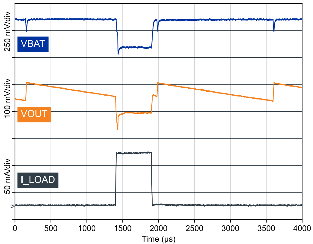
Figure 15: V_{OUT}=1.8\text{ V} : Auto mode load transient from 1\text{ mA} to 100\text{ mA} in 10\text{ }\mu\text{s} (automatic mode change from Low power mode to High power mode, and back)
