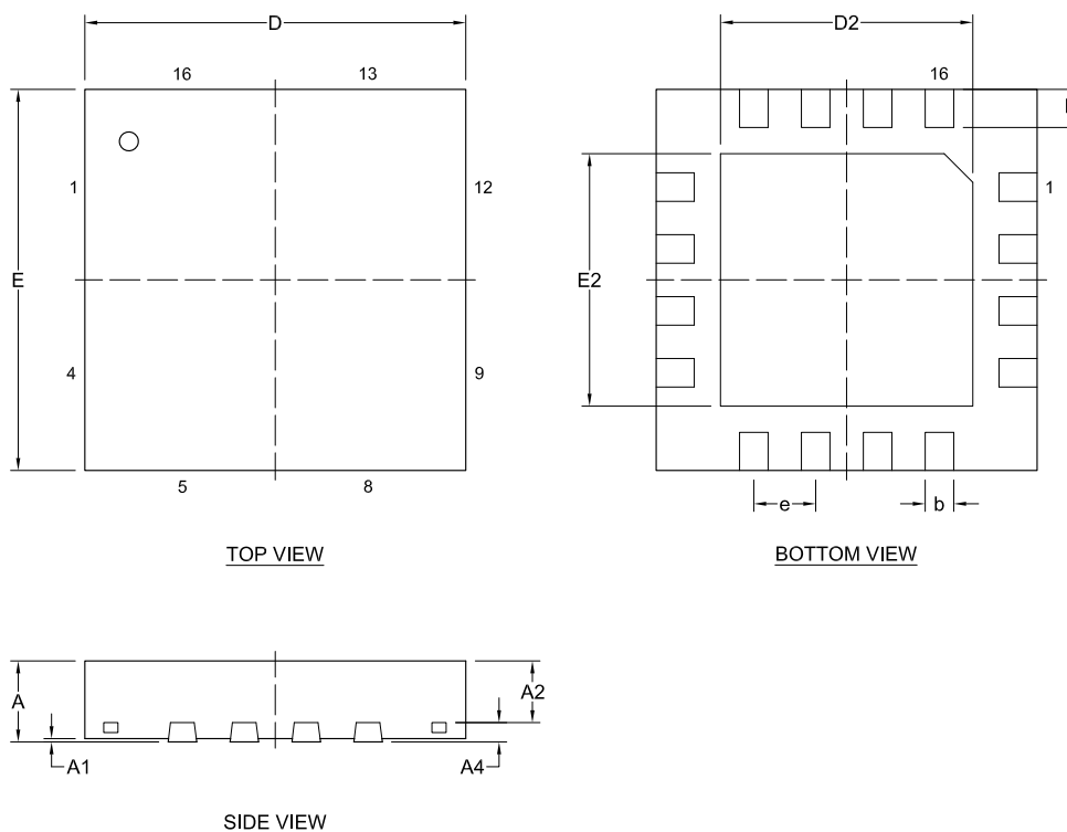
Figure 46: QFN16 4.0x4.0 mm package
