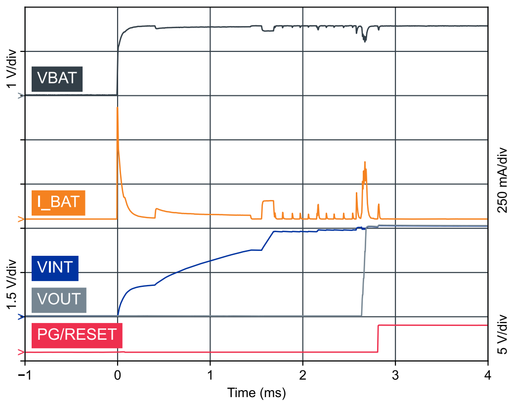
Figure 9: Battery (alkaline AA) insertion, V_{SET} not connected
