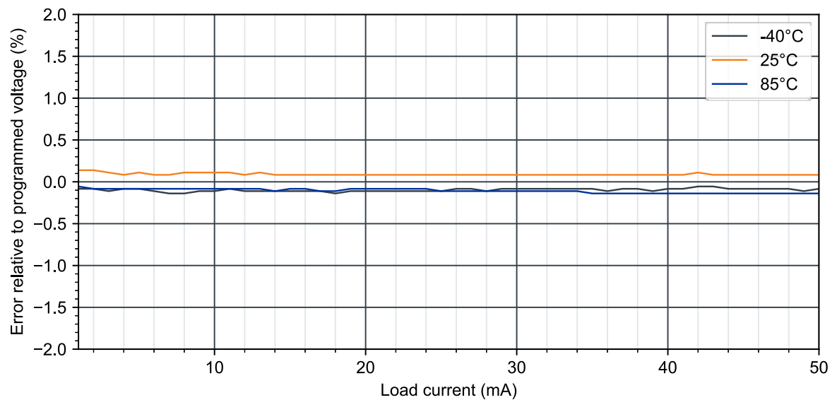
Figure 30: V_{\text{OUTLDO}}=1.8\text{ V} : LDO load regulation in High power mode
