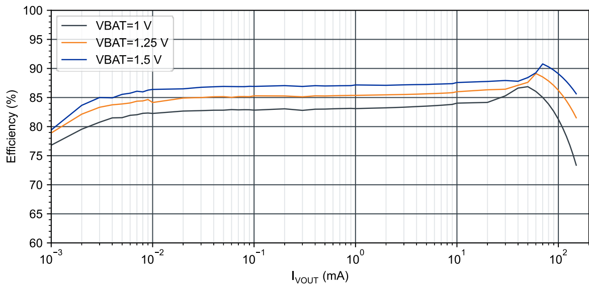
Figure 5: VOUT=1.8 V: Auto mode efficiency
