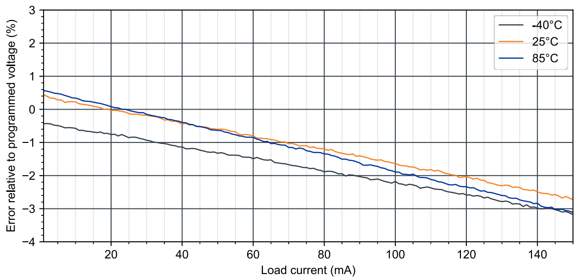
Figure 11: V_{OUT}=1.8 V: High power mode load regulation ( V_{BAT}=1.5 V)
