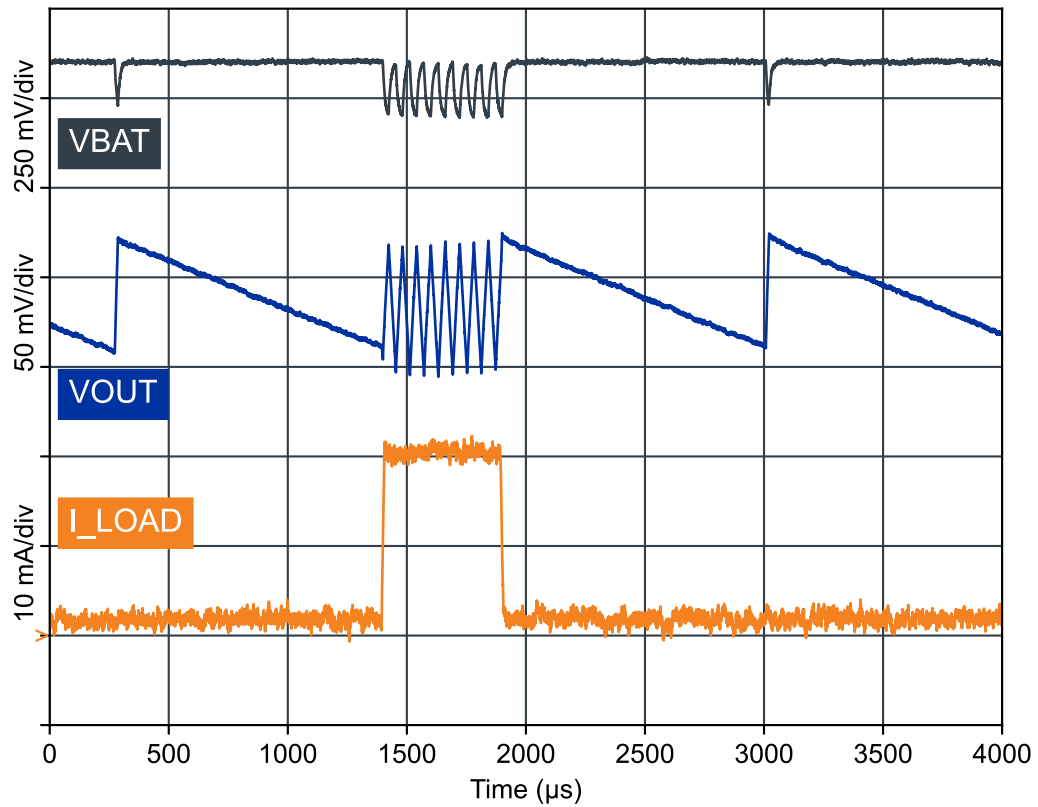
Figure 18: V_{OUT}=3.0 V: Low power mode load transient from 1 mA to 20 mA in 10 µs
