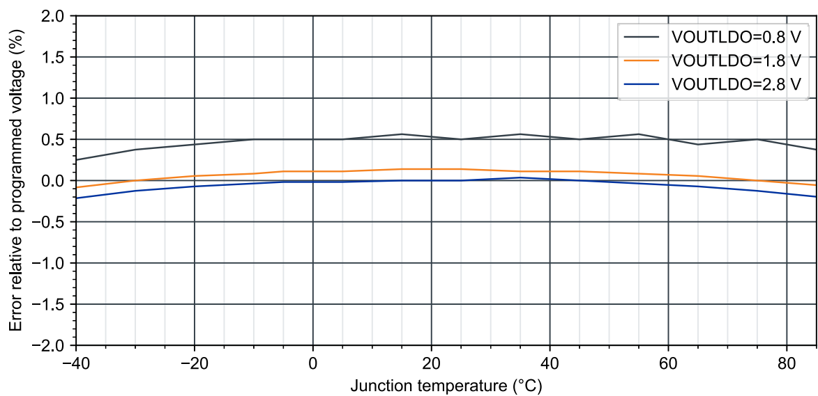
Figure 32: V_{OUTLDO}=1.8\text{ V} : High power mode LDO accuracy over temperature (load=1 mA)
