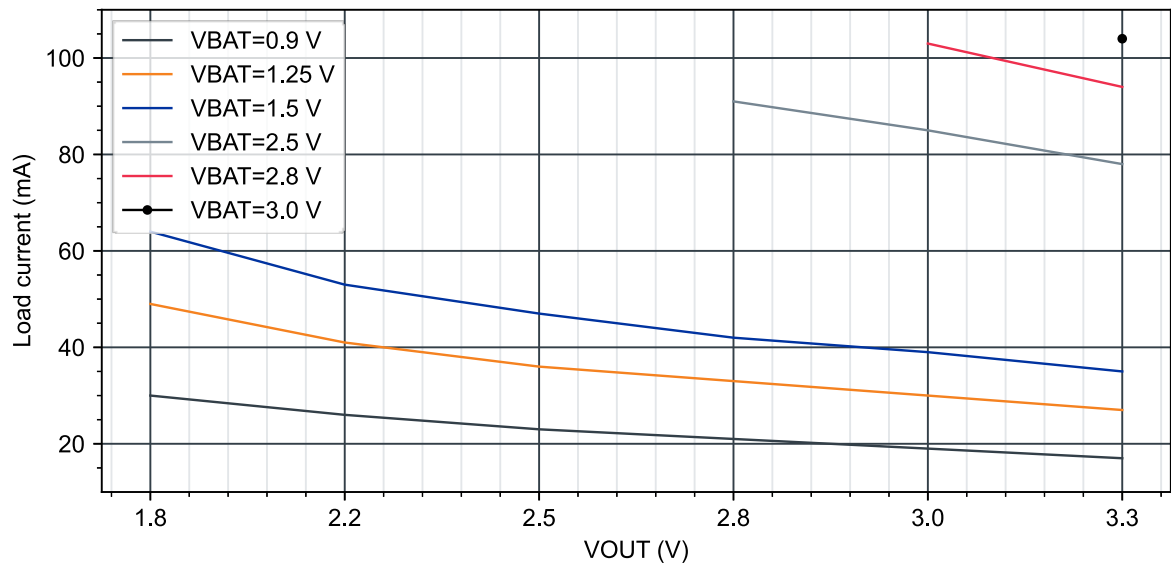
Figure 8: Typical load current vs. V_{OUT} in Auto mode where BOOST changes from Low power mode to High power mode
