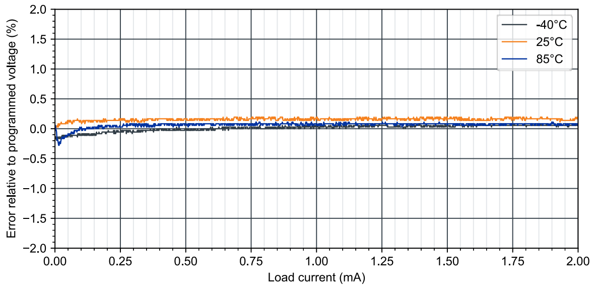
Figure 31: V_{OUTLDO}=1.8\text{ V} : LDO load regulation in Ultra-low power mode
