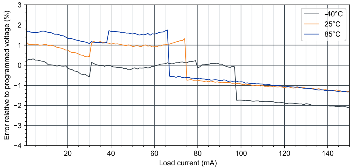
Figure 14: V_{OUT}=3.0\text{ V} : Auto mode load regulation ( V_{BAT}=2.5\text{ V} )
