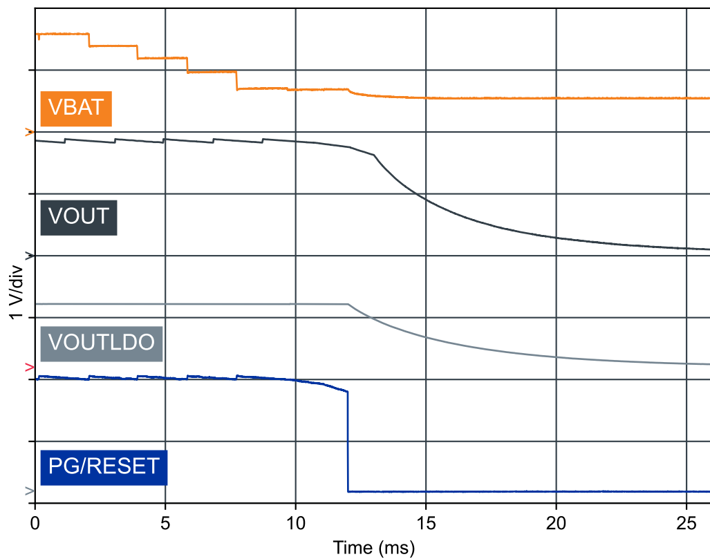
Figure 27: VOUT=1.8 V: battery removal (LDOSW in High power mode, no load)
