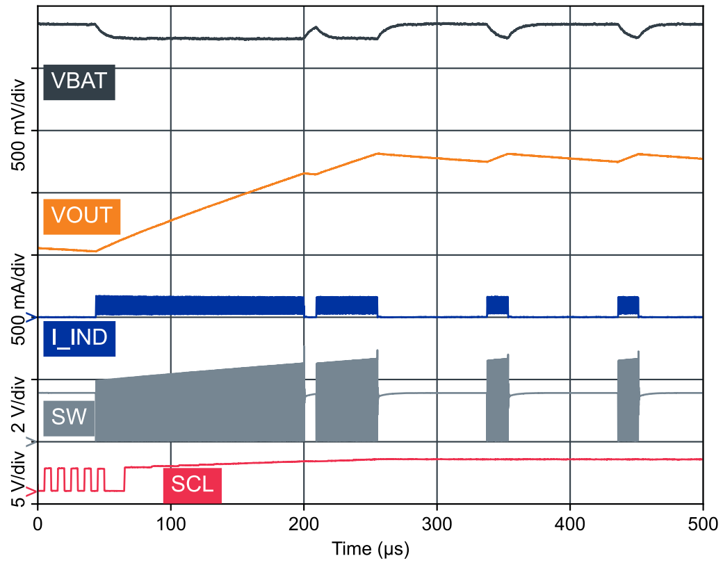
Figure 21: Output voltage programming via TWI from 1.8 V to 2.5 V in Low power mode (LDOSW in High power mode, no load)
