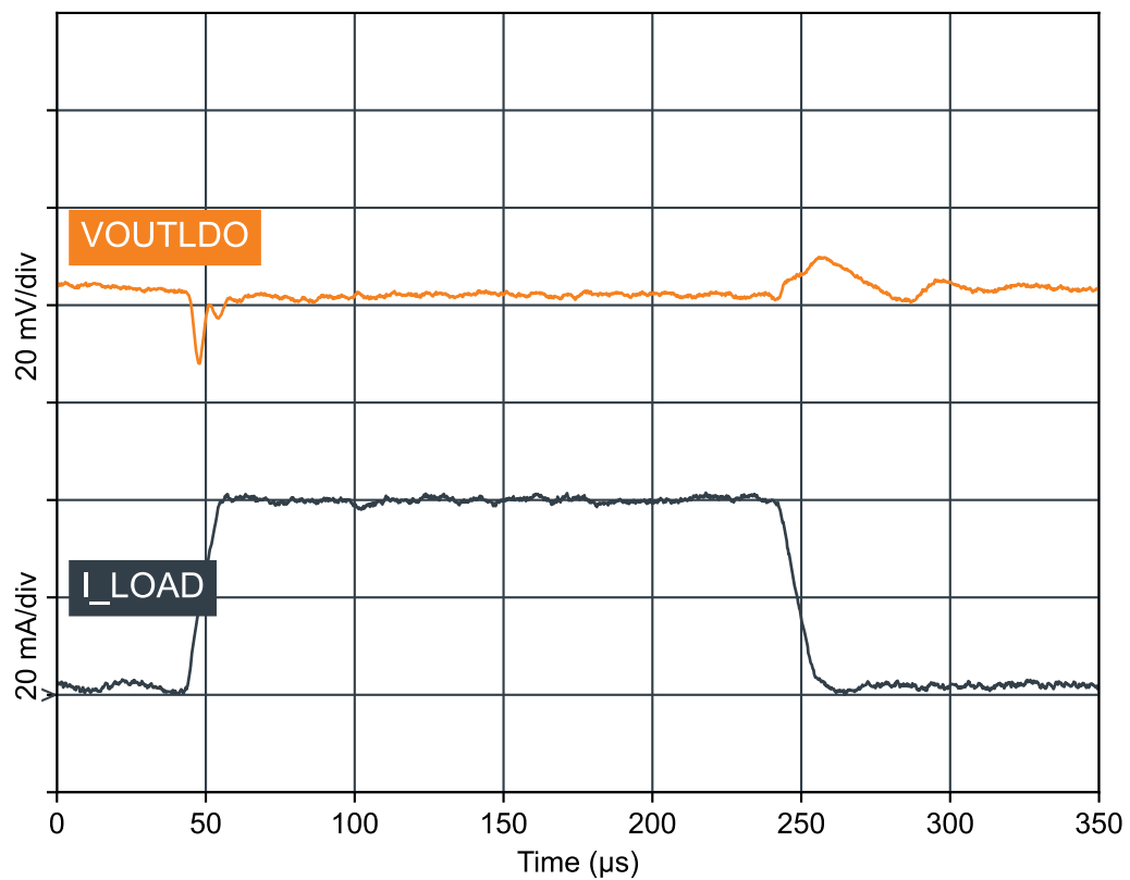
Figure 34: V_{OUTLDO}=1.0\text{ V} : High power mode LDO load transient from 1 mA to 40 mA in 10 \mu\text{s} ( V_{INT}=1.8\text{ V} )
