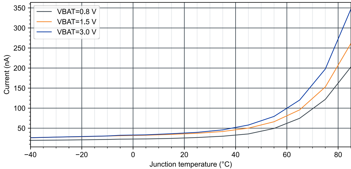
Figure 3: Quiescent current from the battery in Ship mode vs. junction temperature
