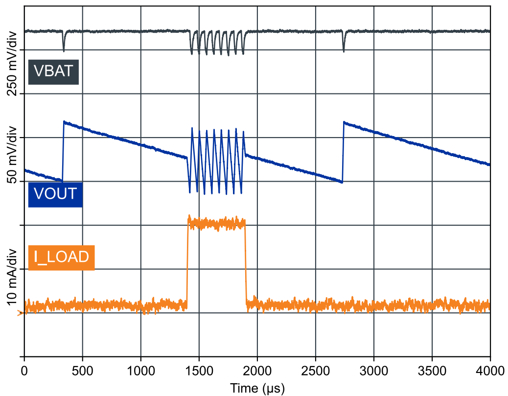
Figure 17: V_{OUT}=1.8\text{ V} : Low power mode load transient from 1 mA to 20 mA in 10 \mu\text{s}
