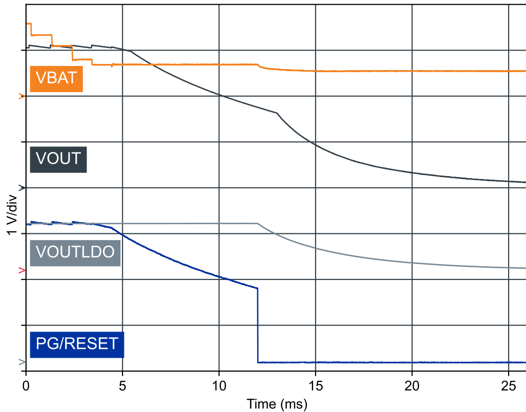
Figure 28: VOUT=3.0 V: battery removal (LDOSW in High power mode, no load)
