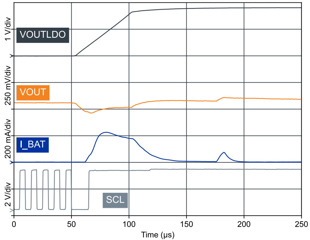
Figure 29: V_{\text{OUTLDO}}=1.8\text{ V} : LDO start-up
