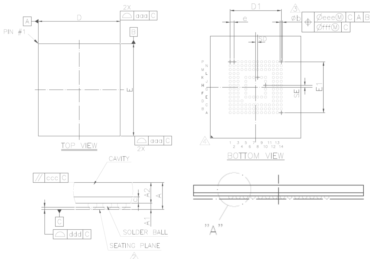
Figure 2 – Package Dimensions
